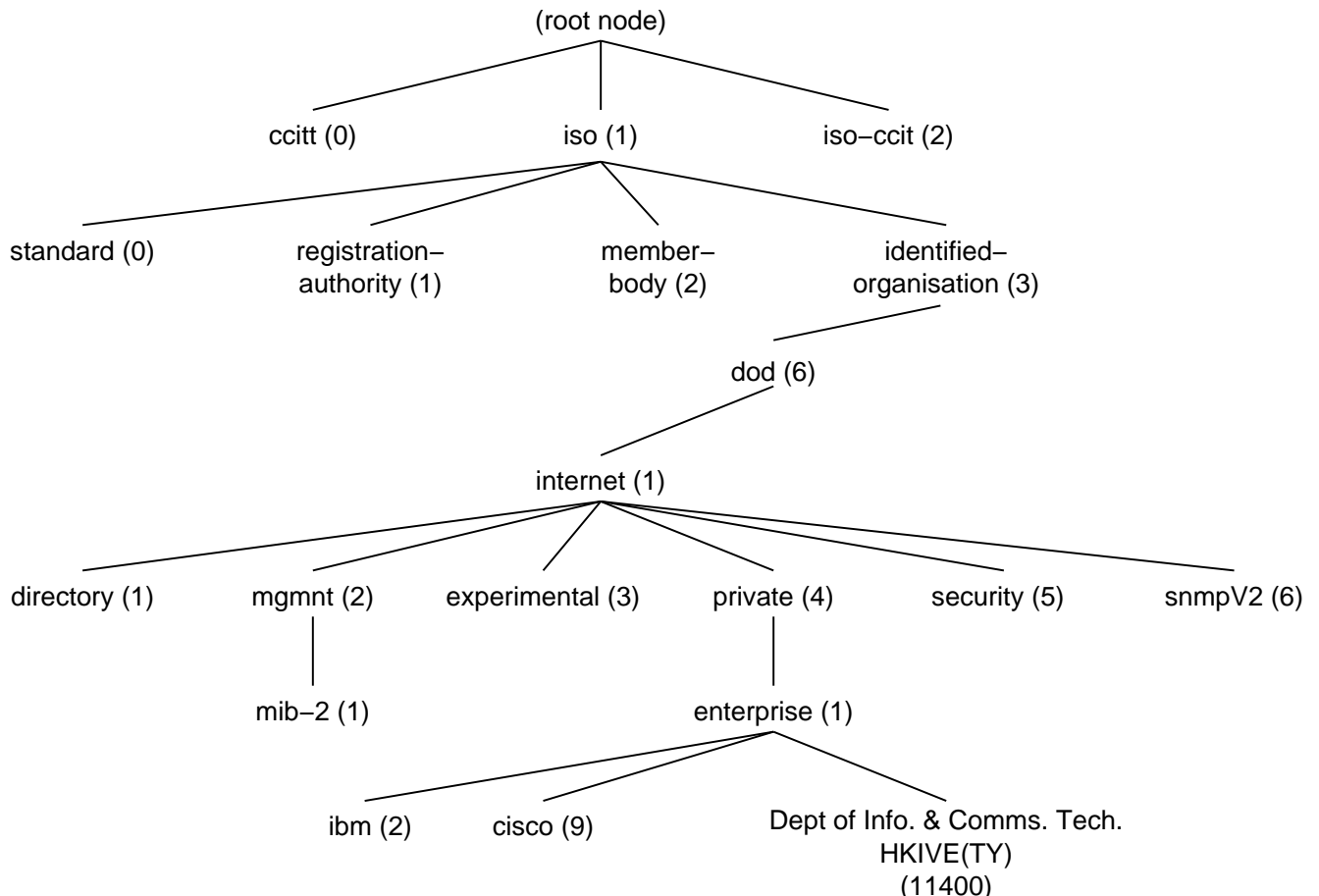
Figure 1: MIB tree.
