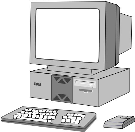
LDAP client
